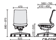
CR-G2900
