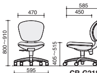
CR-G218
